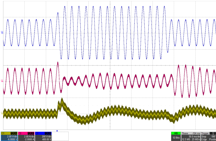
Figure 15: Input voltage transient response with 200µF hold-up capacitor at full load current (115Vrms-230Vrms-115Vrms, 60Hz), Top: Vin (200V/div), Mid: Iin (2A/div), Bottom: Vout (2V/div), Timebase: (50ms/div).
